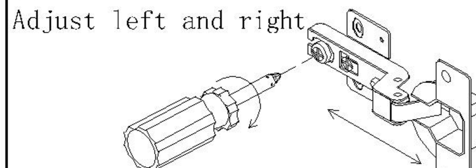
门铰Hinge
