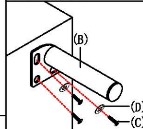
图3: 中脚安装示意图 Figure 3: Middle foot installation diagram
