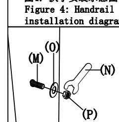
图4: 扶手安装示意图 Figure 4: Handrail installation diagram
